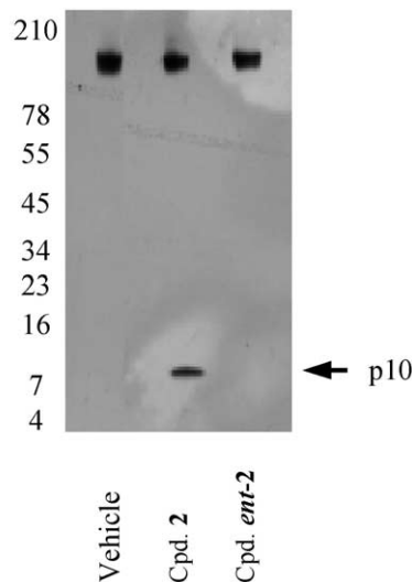
Figure 5. Balb/c male mice were given a single oral dose of 100 mg/kg compound. Splenocytes were collected following dosing, lysed and immunoprecipitated. Western blot analysis for the detection of mouse invariant chain was conducted.
