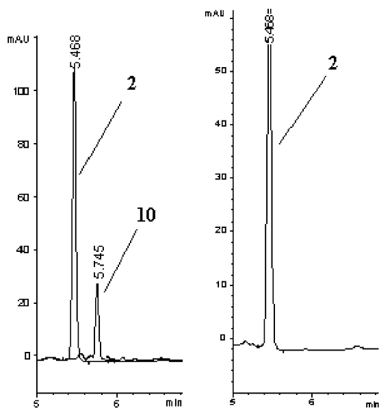
Figure 3. Samples were injected on a 2.1×75 mm, 3.5 \mu m, XDB-C18 column equilibrated in 90% (0.02% phosphoric acid)/10% acetonitrile. A solvent gradient was run to 10% (0.02% phosphoric acid)/90% acetonitrile. Signals were monitored at 254, 280 and 214 nm. Shown are 254 nm signals. Graph A shows the separation of 2 and 10 under these conditions. Graph B is a sample taken from actual in vitro Cathepsin S assay after determining IC_{50} . Graphs A and B show only the region on interest, from 5–6.8 min.
