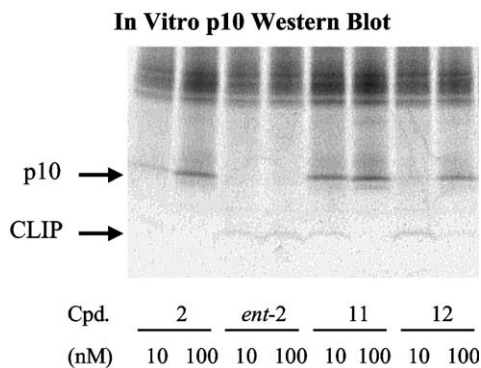
Figure 4. Immunoprecipitation of Class II MHC fragments p10 and CLIP from HOM-2 cells following a 30 min 35 S methionine pulse and 4 h chase in the presence of inhibitors at the concentrations shown.
